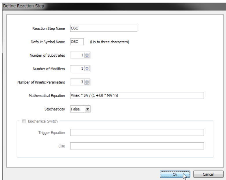
Fig. 6 Define the original mathematical equation and customize this equation as the user-defined reaction step symbol (called OSC in this case). The customized reaction step symbol appears in the Symbol Selection area.
