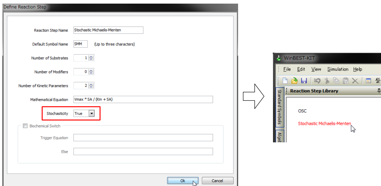
Fig. 7 Define the Michaelis-Menten equation which involves with the stochastic fluctuation and customize this equation as the user-defined reaction step symbol (called Stochastic Michaelis-Menten in this case). The customized reaction step symbol appears in the Symbol Selection area.
